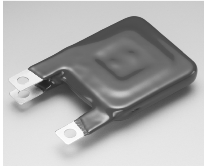
Dual Disc Device - Two 34mm varistor discs in parallel in a single package
