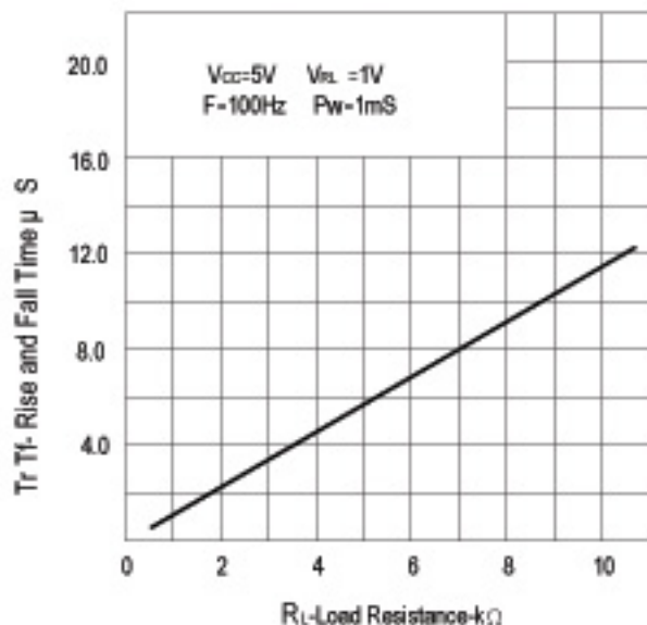
FIG.3 RISE AND FALL TIME VS. LOAD RESISTANCE
