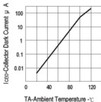
FIG.1 COLLECTOR DARK CURRENT VS. AMBIENT TEMPERATURE
