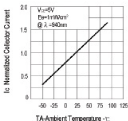
FIG.2 NORMALIZED COLLECTOR CURRENT VS. AMBIENT TEMPERATURE
