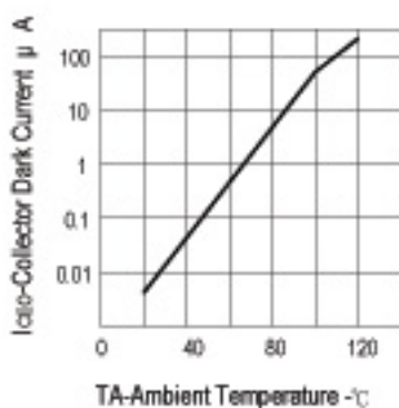
FIG.1 COLLECTOR DARK CURRENT VS. AMBIENT TEMPERATURE
