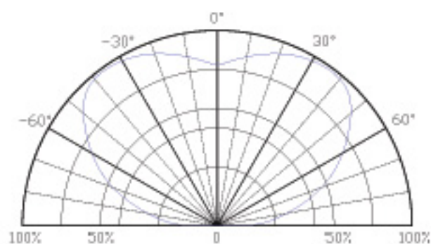
View angle 150° (2θ 1/2)
