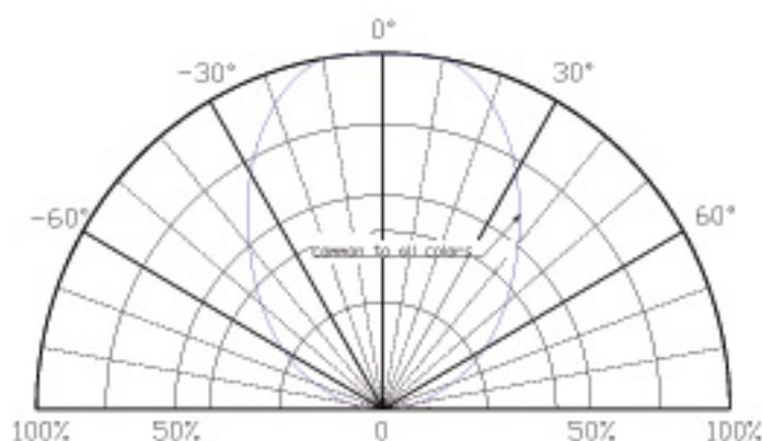
View angle 80° (2θ 1/2)
