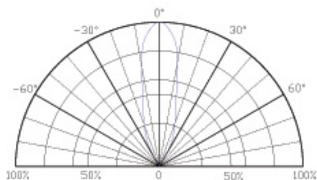
View angle 20° (2θ 1/2)
