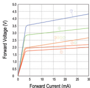
Forward Voltage vs. Forward Current
