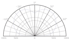
View angle 150° (2 θ 1/2)
