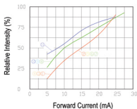
Relative Intensity vs. Forward Current
